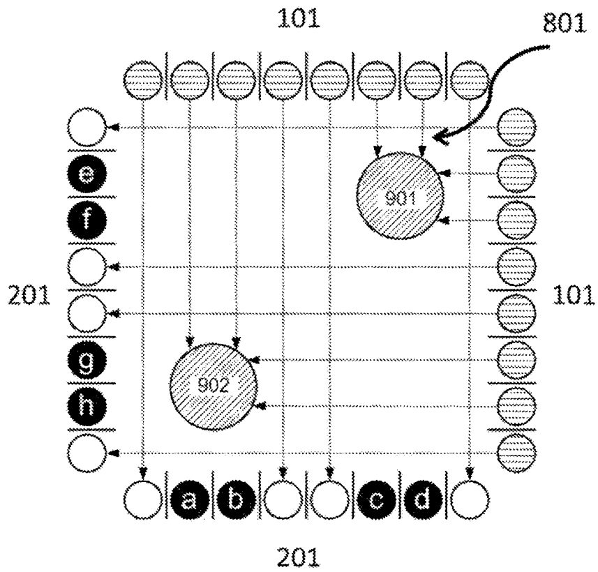
FIG. 3 (PRIOR ART)
